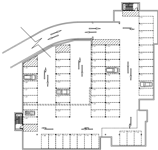
BASEMENT LEVEL PLAN
